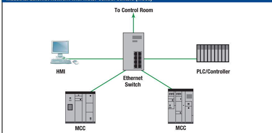
Industrial Ethernet Network with Motor Control Centers (MCCs)
